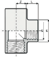
T12 90° Tee with BSP threaded female ends
