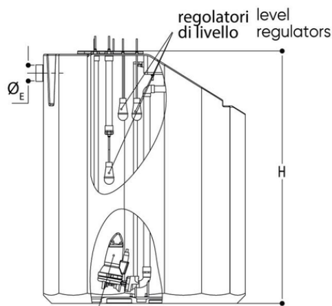
elettropompa sommersibile submersible motor-driven pump
